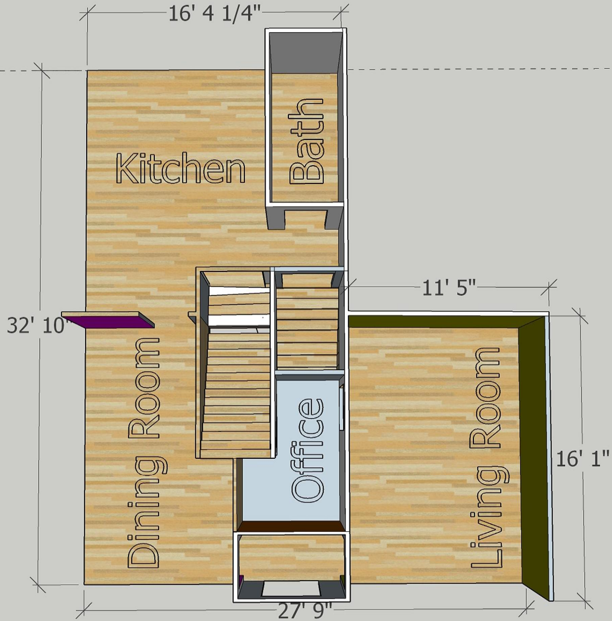
Before - 1st Floor Plan 81 Sacramento Street
